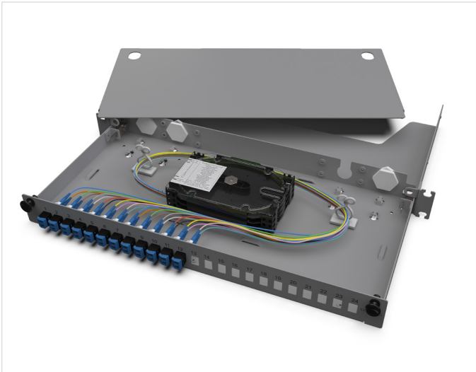
Everon LAN1 Fibre Housing with Adapters, splice pack, grey | Photo REN10027
