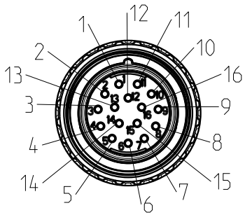
socket face female
