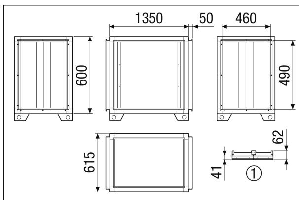
1 Detail Dach
