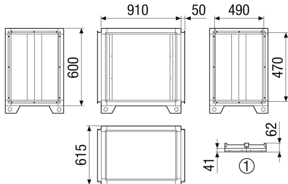
1 Detail Dach
