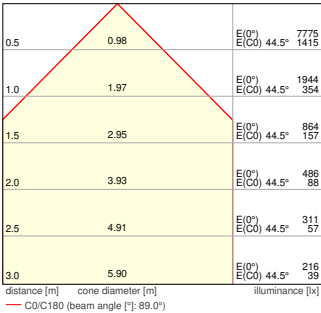
PL CMFT 625 P 30W ML 840 U19 With Circular Cut Out
