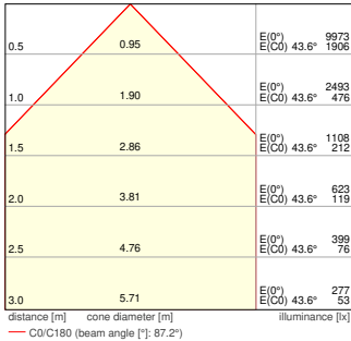
PL CMFT 625 P 30W ML 840 U19 With Inverted Frame
