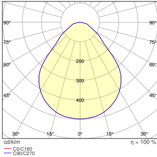
PL CMFT 625 P 30W ML 840 U19 With Inverted Frame
