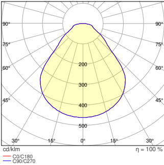
PL CMFT 625 P 30W ML 840 U19 With Circular Cut Out
