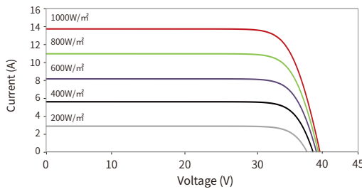
Current-Voltage Curves (54HL4R-B 445W)
