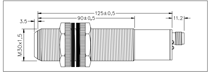
Dimensions/Abmessungen/Dimensions
