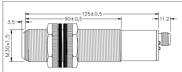
Dimensions/Abmessungen/Dimensions
