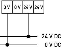
Wiring diagram of the alarm contacts
