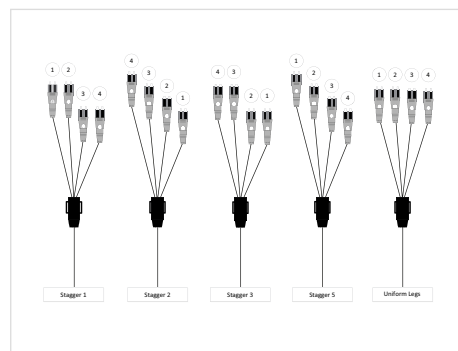
EDGE8 Staggered Harness Examples | Photo ZA4253
