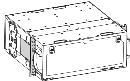
Housing ready for installation with a 3-in projection from frame
