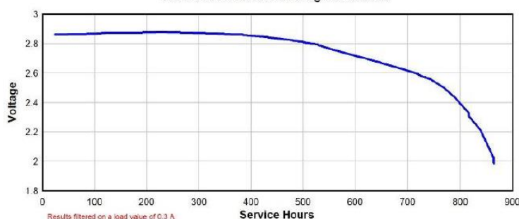
Low Load Pulse Test 300mA Pulse with 2mA Background to 1.8V
