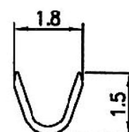
B-B SECTION
