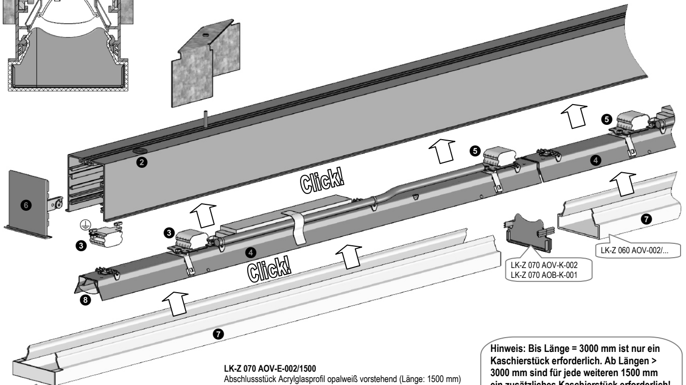
LK-Z 070 AOV-E-002/1500
