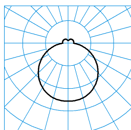
Solegra WD2 OTA 6000-830 + WD2 ZPF-T C1/C TX062810
