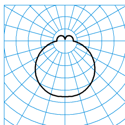
Solegra WD1 OTA 2600-830 + ZS A 3075/1500 TX062854 UGR I = 20.5 UGR q = 20.5 DIN 5040: B31 UTE: 0,81 G + 0,19 T CEN Flux Code: 40 70 90 81 100 19 45 72 19 ■ C0 - C180 ■ C90 - C270
