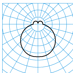
Solegra WD1 OTA 2600-830 + WD1 ZPF-T C1/C TX062853 UGR I = 20.5 UGR q = 20.5 DIN 5040: B31 UTE: 0,81 G + 0,19 T CEN Flux Code: 40 70 90 81 100 19 45 72 19 ■ C0 - C180 ■ C90 - C270
