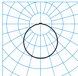
Olisq Act RWD4 DW 40 ETDD8 IP54 (ActDCW) TX375934
