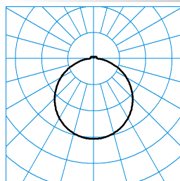
Olisq Act RWD4 DW 40 ETDD8 IP54 (ActDWW) TX375939
