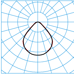
Belviso C2 600 CDP LED3800nw FB TX037977
