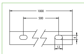
Abb. 1 Position der Schlitze Pic. 1 Needlepoints position
