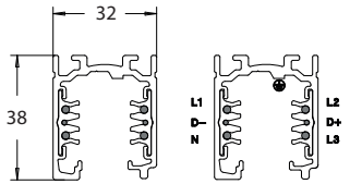
Anbauschiene ST-A... Surface-mounted track ST-A...
