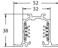
Anbauschiene ST-A... Surface-mounted track ST-A...
