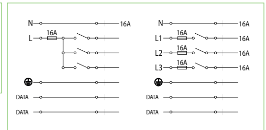
Abb. 3 Schaltplan Pic. 3 Electrical scheme
