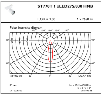
OFPC1_ST770T1xLED27S830HMB
