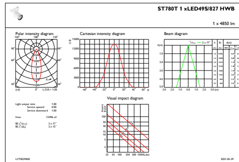
IFAS1_ST780T1xLED49S827HWB
