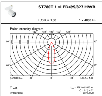
OFPC1_ST780T1xLED49S827HWB
