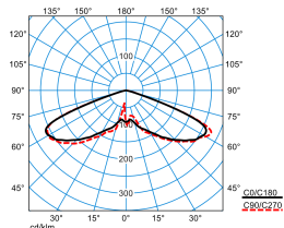
Publisca P1-RB6L/2600-730 3G1S ETDD (CLO end value)
