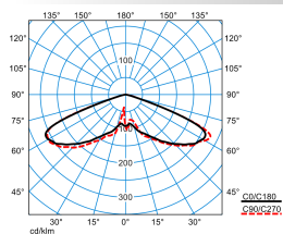
Publisca P1-RB6L/2600-730 3G1S ETDD (CLO initial value)
