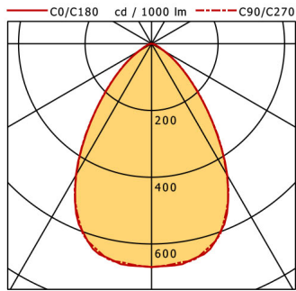
Flixx 200 Square (FLIQZ 200.05, 1xLED 27W 827/2700K 2540lm 70 °)
