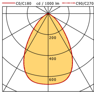
Flixx 200 Square (FLIQZ 200.05, 1xLED 27W 827/2700K 2540lm 70 °)
