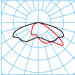
LnPlus 60-AB7L-LR/26000-727 24G1 ET (CLO initial value) TX390201 ■ C0 - C180 ■ C90 - C270 DIN 5040: A30 UTE: 1,00 G CEN Flux Code: 35 73 98 100 100
