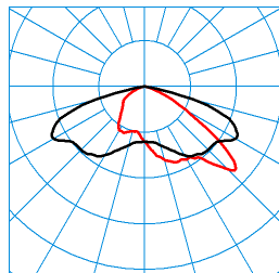
LnPlus 60-AB7L/20000-722 24G1 ETDD (CLO initial value) TX377545 DIN 5040: A30 UTE: 1,00 G CEN Flux Code: 35 73 98 100 100 ■ C0 - C180 ■ C90 - C270
