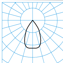
Faciella Slim 40 RB20R/7600-830 6G1 TX120354
