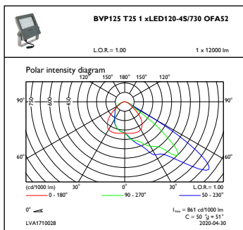
OFPC1_BVP125T251xLED120-4S730OFA52
