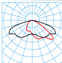
LIQ 70N-AB7L-LR/10000-727 12G1 ET(CLO end value) TX278264 DIN 5040: A30 UTE: 1,00 G CEN Flux Code: 35 73 98 100 100 0 0 0 0 ■ C0 - C180 ■ C90 - C270
