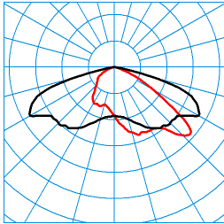
LIQ 70N-AB7L-LR/9100-727 10G1 ET (CLO initial value) TX278097 ■ C0 - C180 ■ C90 - C270 DIN 5040: A30 UTE: 1,00 G CEN Flux Code: 35 73 98 100 100 0 0 0 0
