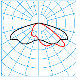
LIQ 70N-AB7L-LR/9100-727 10G1 ET (CLO end value) TX278012 ■ C0 - C180 ■ C90 - C270 DIN 5040: A30 UTE: 1,00 G CEN Flux Code: 35 73 98 100 100 0 0 0 0
