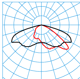
LIQ 70N-AB7L-LR/7500-727 8G1 ET(CLO initial value) TX277973 DIN 5040: A30 UTE: 1,00 G CEN Flux Code: 35 73 98 100 100 0 0 0 0 ■ C0 - C180 ■ C90 - C270
