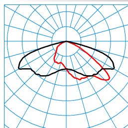
LIQ 70N-AB7L-LR/6800-727 8G1 ET(CLO end value) TX277774 DIN 5040: A30 UTE: 1,00 G CEN Flux Code: 35 73 98 100 100 0 0 0 0 ■ C0 - C180 ■ C90 - C270
