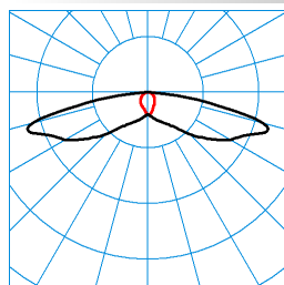
LIQ 50N-SB3L-LR/1350-727 2G1 ET (CLO end value) TX278109 DIN 5040: A30 UTE: 1,00 l CEN Flux Code: 31 64 92 100 100 ■ C0 - C180 ■ C90 - C270
