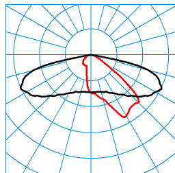
LIQ 50N-AB2L-SLR2/2200-727 2G1 ET(CLO initial value) TX278167 DIN 5040: A30 UTE: 1,00 G CEN Flux Code: 34 71 96 100 100 0 0 0 0 ■ C0 - C180 ■ C90 - C270
