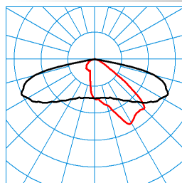
LIQ 50N-AB2L-LR/1350-727 2G1 ET(CLO end value) TX278026 DIN 5040: A30 UTE: 1,00 G CEN Flux Code: 34 71 96 100 100 0 0 0 0 ■ C0 - C180 ■ C90 - C270
