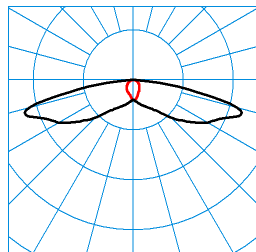
LIQ 50N-SB3L-LRA/1800-727 2G1 ETDD(CLO initial value) TX278211 DIN 5040: A30 UTE: 1,00 l CEN Flux Code: 31 64 92 100 100 ■ C0 - C180 ■ C90 - C270
