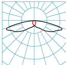
LIQ 50N-SB3L-LRA/1500-727 2G1 ETDD(CLO initial value) TX277810 DIN 5040: A30 UTE: 1,00 l CEN Flux Code: 31 64 92 100 100
