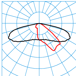
LIQ 50N-AB2L-LRA/3500-727 4G1 ETDD(CLO initial value) TX278294 DIN 5040: A30 UTE: 1,00 G CEN Flux Code: 34 71 96 100 100 0 0 0 0
