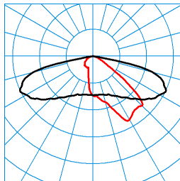
LIQ 50N-AB2L-LRA/3500-727 4G1 ETDD(CLO end value) TX277843 DIN 5040: A30 UTE: 1,00 G CEN Flux Code: 34 71 96 100 100 0 0 0 0
