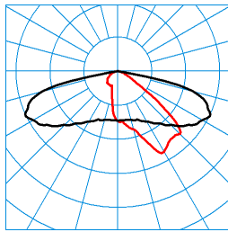
LIQ 50N-AB2L-LRA/22/26/32-722 4G1 (CLO end value 0) TX280926
