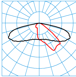
LIQ 50N-AB2L-LRA/22/26/32-722 4G1 (CLO end value 2) TX280945
