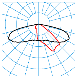
LIQ 50N-AB2L-LRA/22/26/32-722 4G1 (CLO initial value 1) TX280995
