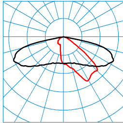
LIQ 50N-AB2L-LRA/22/26/32-722 4G1 (CLO end value 1) TX281120
