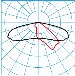
LIQ 50N-AB2L-LRA/22/26/32-722 4G1 (CLO initial value 2) TX281140
