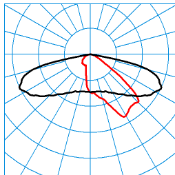
LIQ 50N-AB2L-LRA/22/26/32-722 4G1 (CLO initial value 0) TX280881
