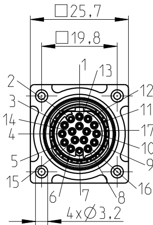
socket face female
