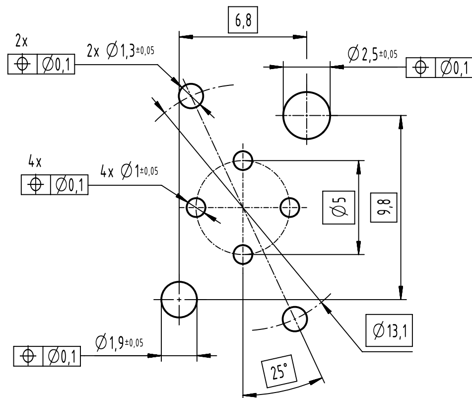
recommended PCB-layout A (5:1)
