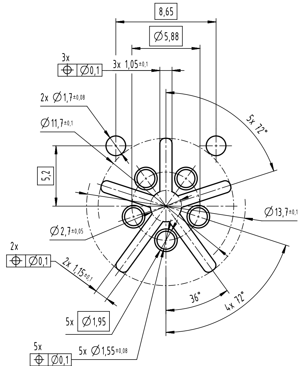
recommended PCB-layout A (5:1)
