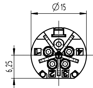
view without pick & place cap
