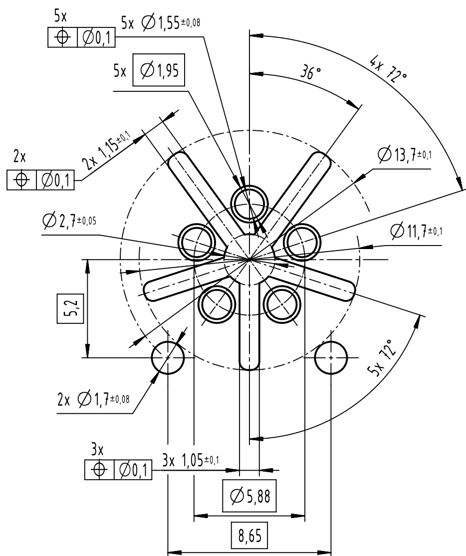
recommended PCB-layout A (5:1)
