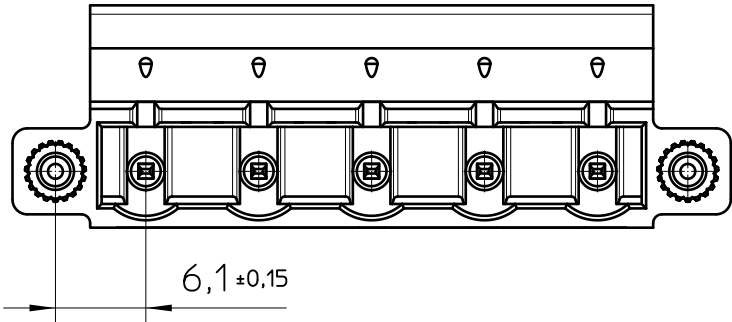
view "X"
