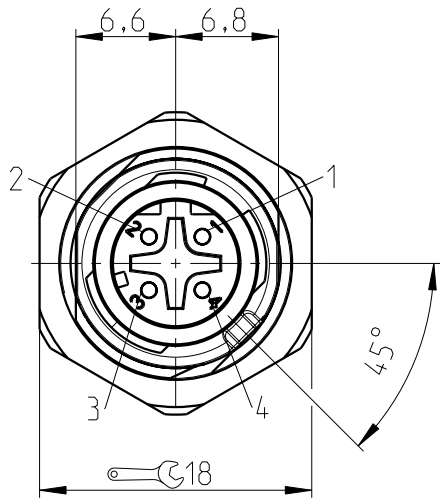
plug face male
