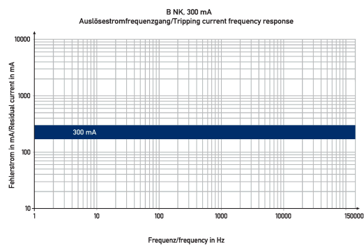
Diagramme FI-/LS-Kombinationen DRCBO 4 B20/o,30/3N-B NK
