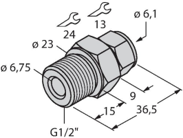
CF-M-6-G1/2-A4 9910530
