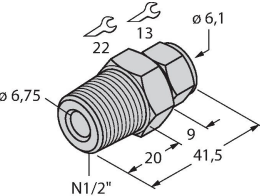
CF-M-6-N1/2-A4 9910529
