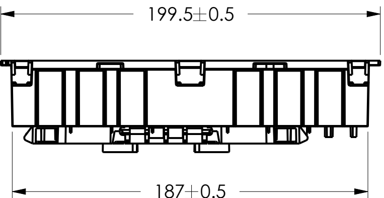
VIEW VB
